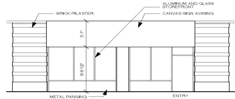
EXTERIOR ELEVATION 0 1 3 4 5 6 8 9 10 FT
